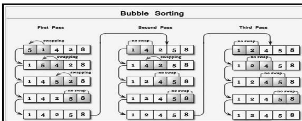
Fig.17.1 Bubble Sort
