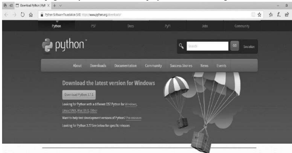
Fig.1.1: Home Page
